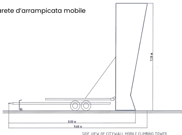
SIDE VIEW OF CITYWALL MOBILE CLIMBING TOWER
